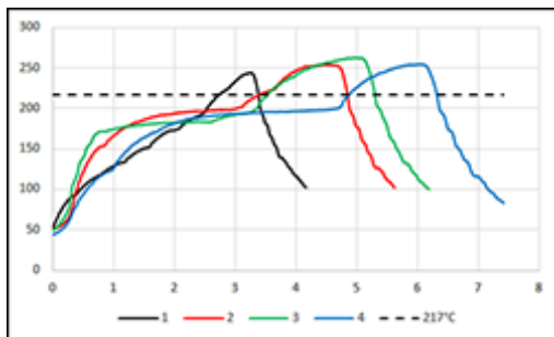
Reflow Profile
